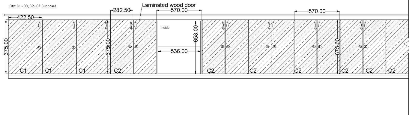
Drawing - 2 Front view
